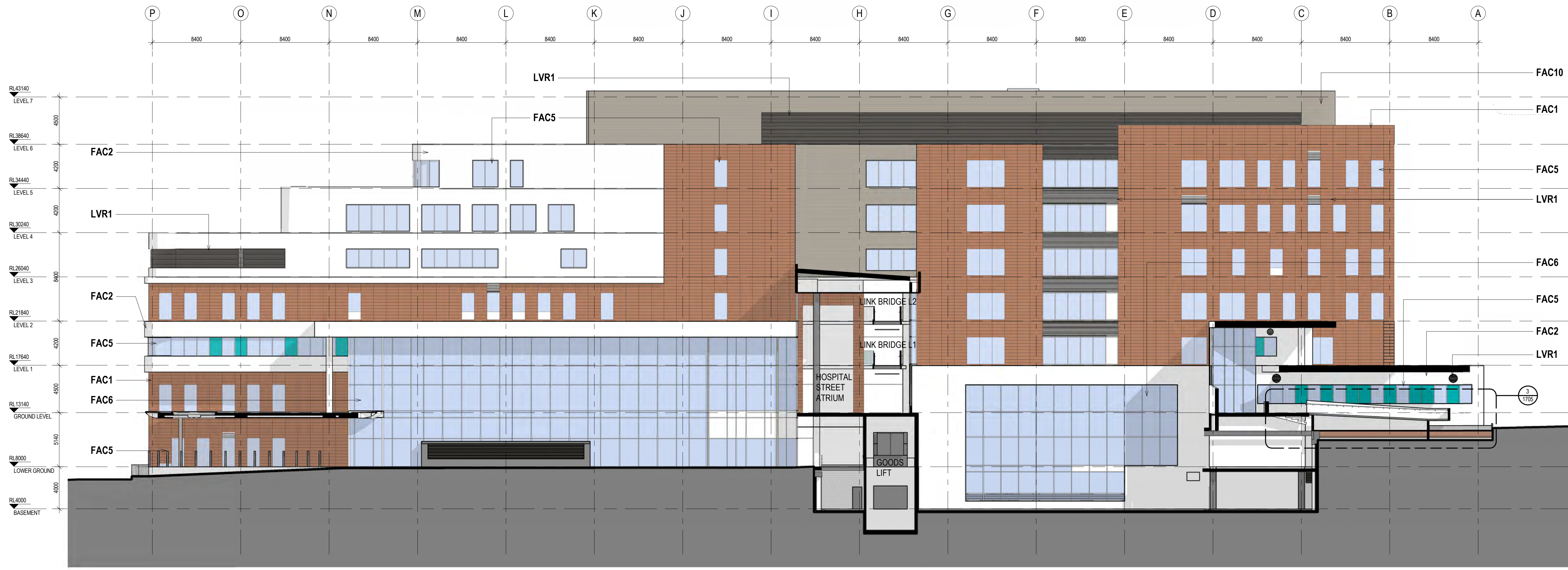
1 NORTH ELEVATION / SECTION 15B2 1:200
